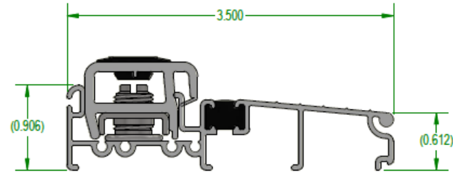
VIEW2 SCALE 1 : 1
