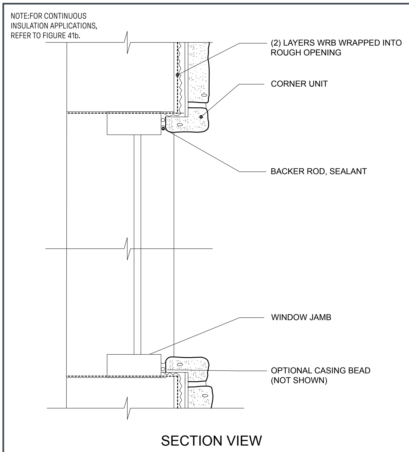
Figure 42. Forward Mounted Commercial Window – Top View
