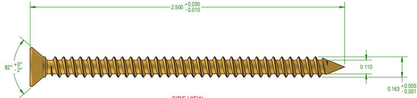
SIDE VIEW SCALE 3 : 1
