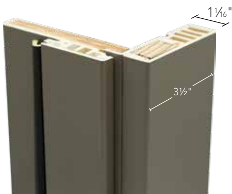
3 ½" FLAT RIPPABLE BRICKMOLD
