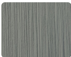
Granite
